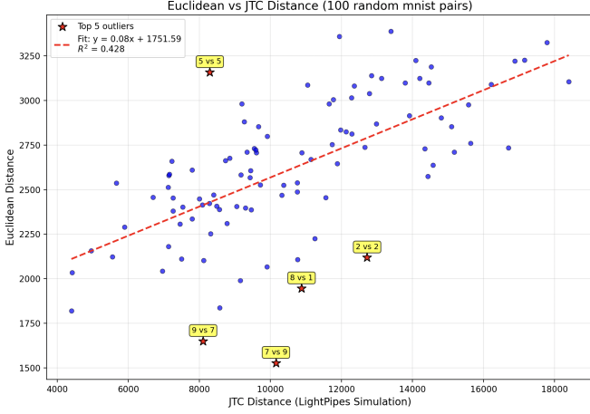
Figure 4: Scatter plot of the JTC dissimilarity versus the Euclidean distance for 100 random pairs of MNIST digits. The coefficient of determination is R^2 = 0.428 . While the R^2 value is relatively low, multiple outliers contribute to this reduction. However, the general trend of the data is well captured by the fitted line, indicating a meaningful correlation between JTC dissimilarity and Euclidean distance.
